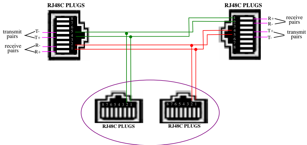
Figure 2-7 Deployment of Monitored Lines
