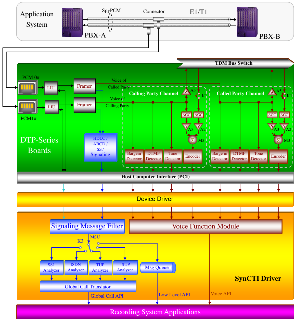
Figure 1-1 Operation Principle
