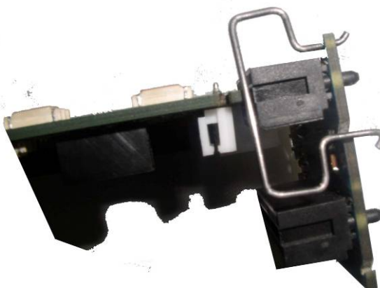
Figure 2-15 Insertion of Motherboard
