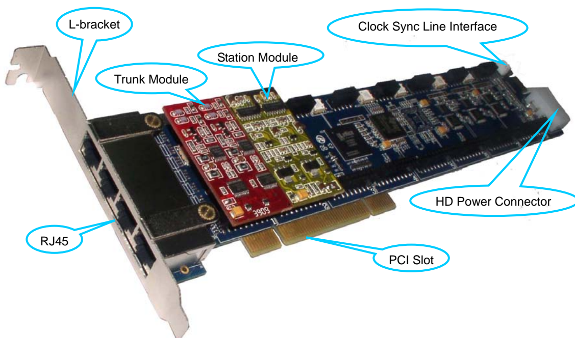
Figure 2-2 FXM3210P Motherboard
