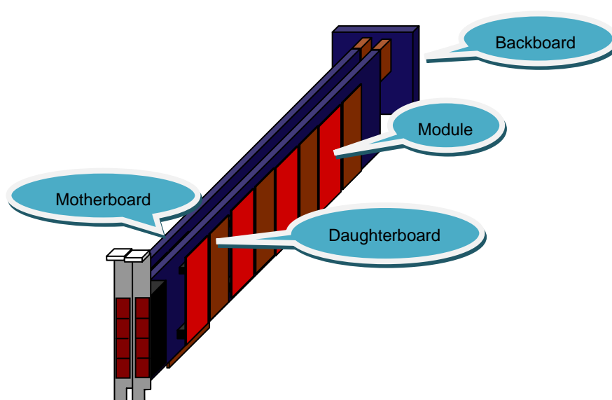
Figure 2-1 Overall Structure
