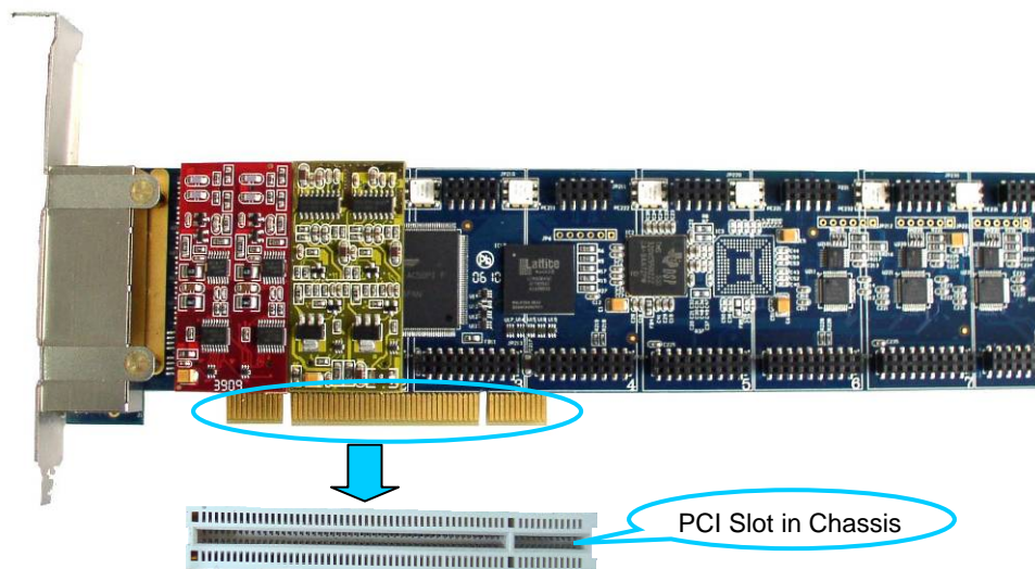
Figure 2-8 Insert Motherboard to PCI/PCIe Slot
