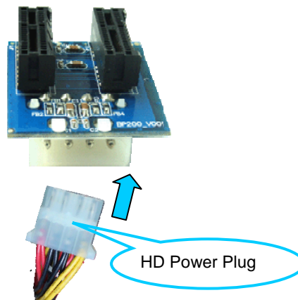
Figure 2-9 Fit HD Power Plug to Backboard
