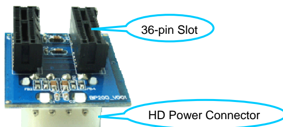
Figure 2-3 BP200 Backboard
