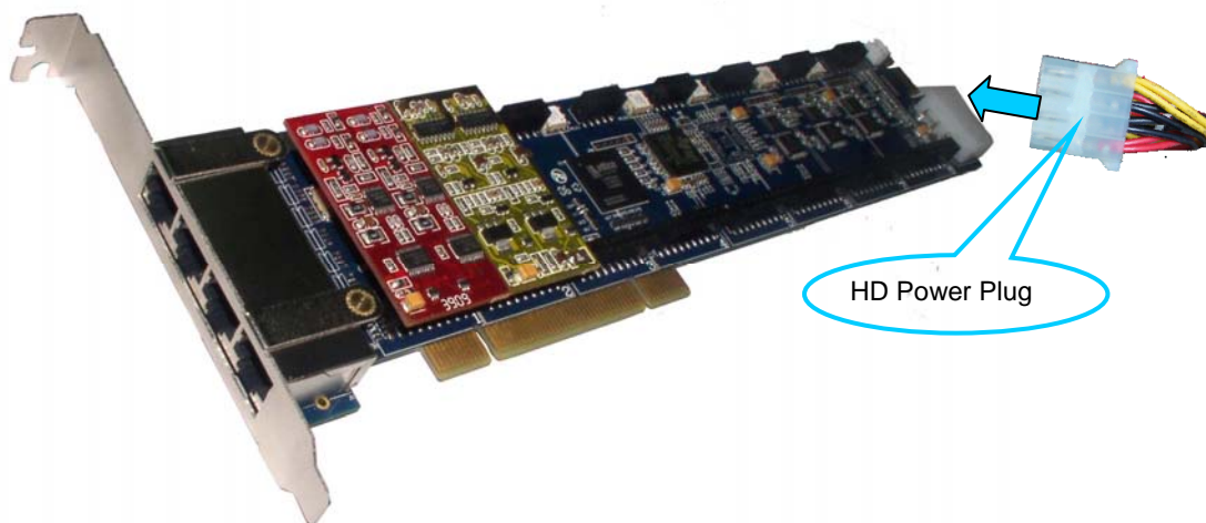
Figure 2-10 Fit HD Power Plug to Motherboard
